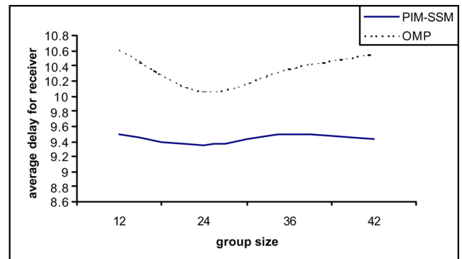
Figure 16 Delay for receiver in traceroute topology (PIM-SSM vs. OMP) (see online version for colours)
