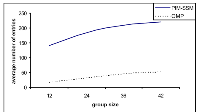
Figure 5 Table size in traceroute topology (PIM-SSM vs. OMP) (see online version for colours)
